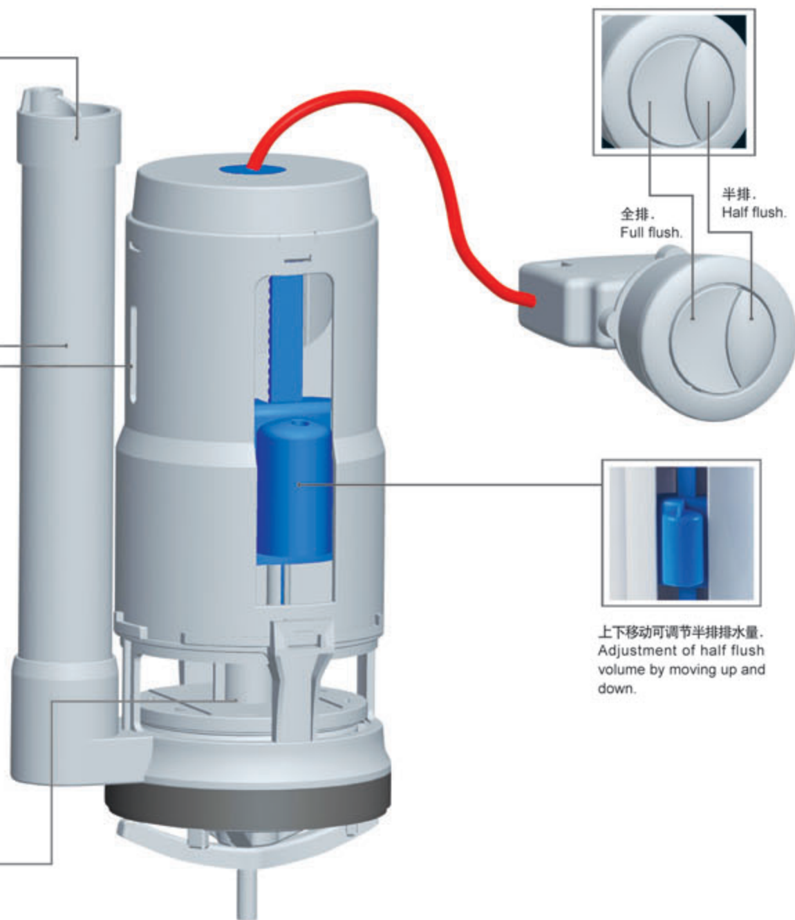
可选不同高度的溢水管。 Overflow pipe is available in any height.
